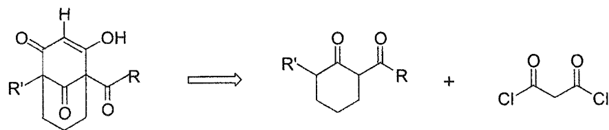
Figure 5. Retrosynthetic Analysis
